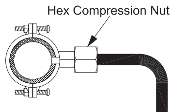
Figure 2: Drain Saddle Assembly Sequence
