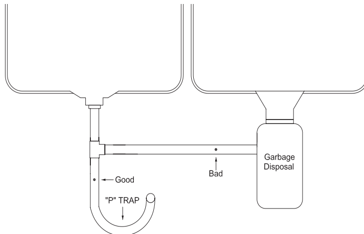
Figure 1: Drain Saddle Mounting Locations
